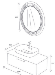
Antique White BANYO DOLABI BATHROOM CABINET KOD/CODE W012.100.102
